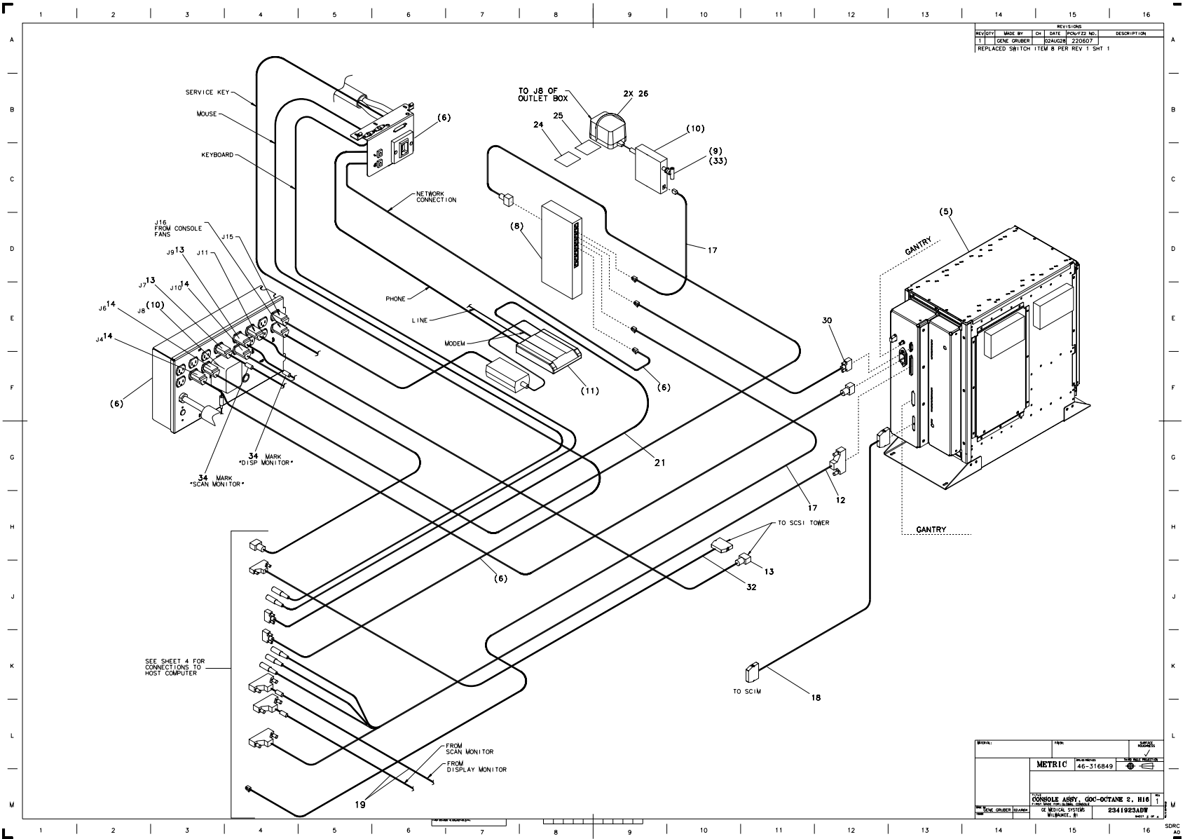
Figure 5-4 Console (2341923, sheet 3, rev 1)
