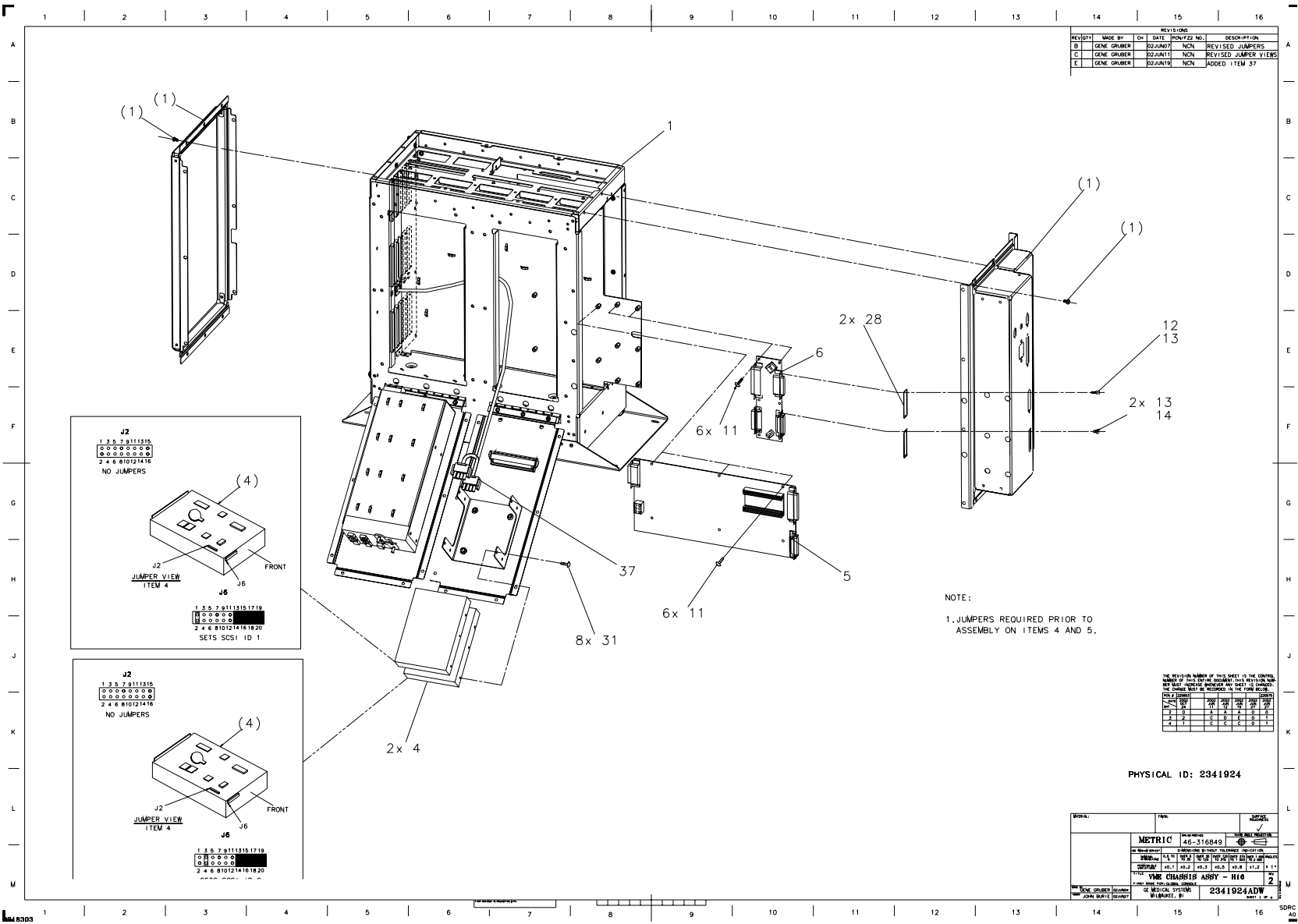
Figure 5-9 Recon Box Assembly (2341924, sheet 1, rev 2)
