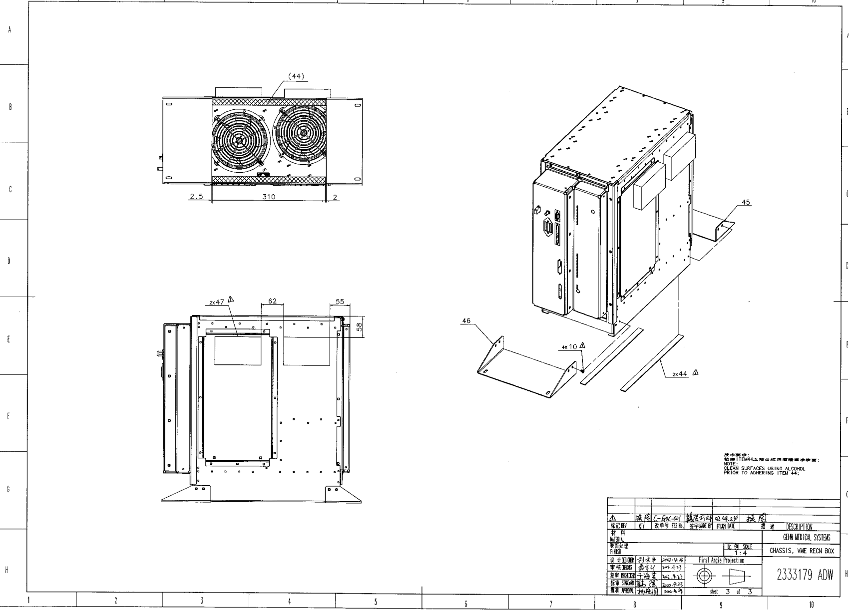
Figure 5-15 VME Recon Box Chassis (2333179 sheet 3, rev 1)
