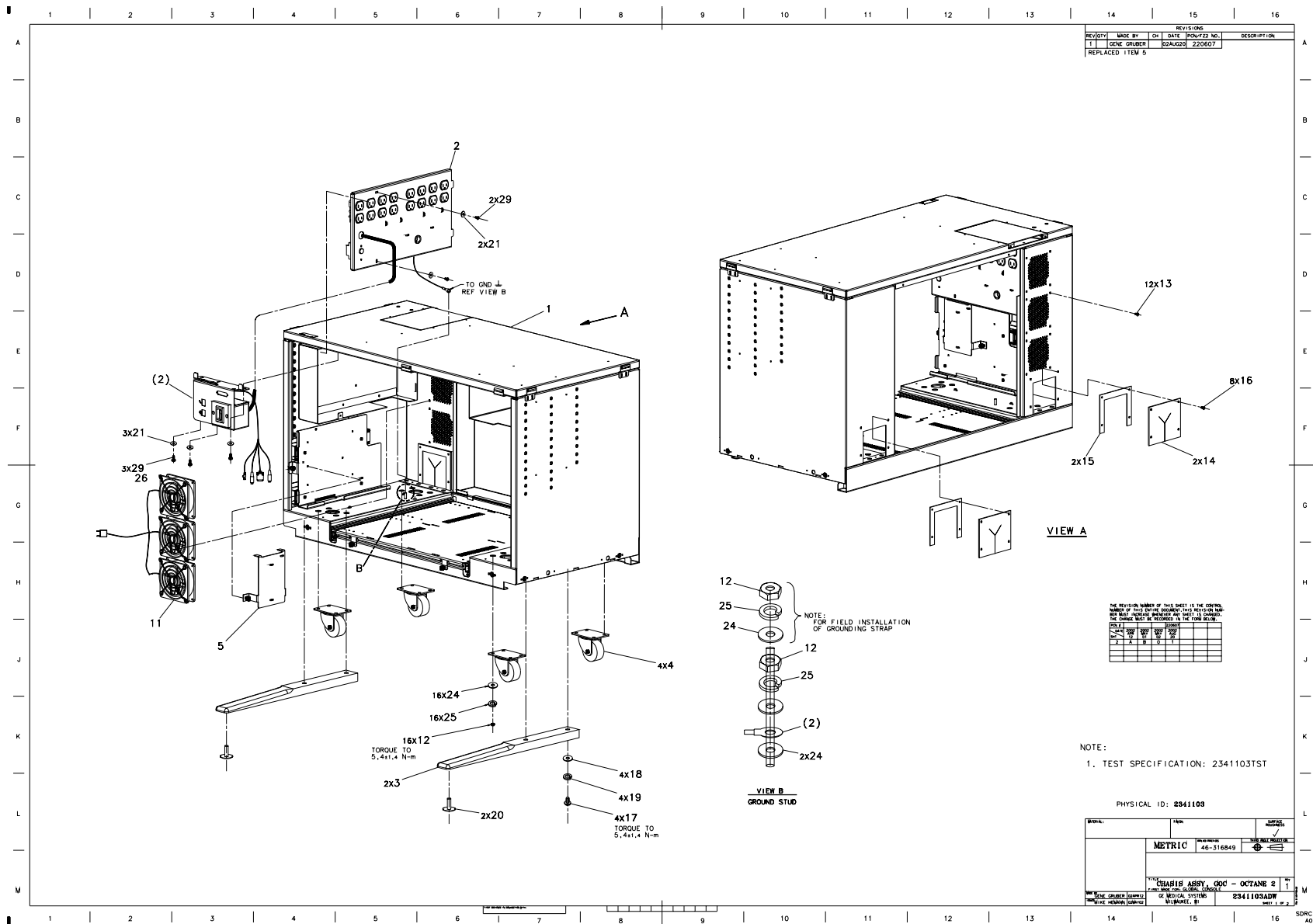
Figure 5-26 Console Chassis Assembly (2341103, sheet 1, rev 1)
