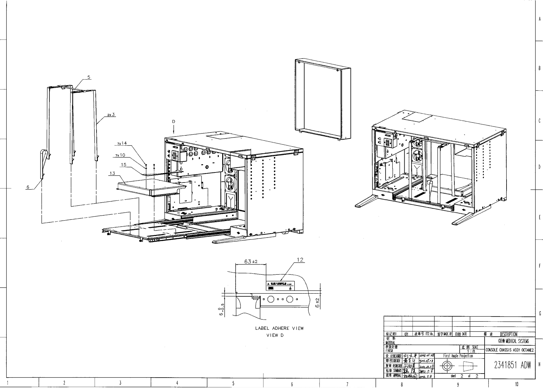
Figure 5-22 Console Chassis Assembly, Octane2 (2341851 sheet 2, rev 0)
