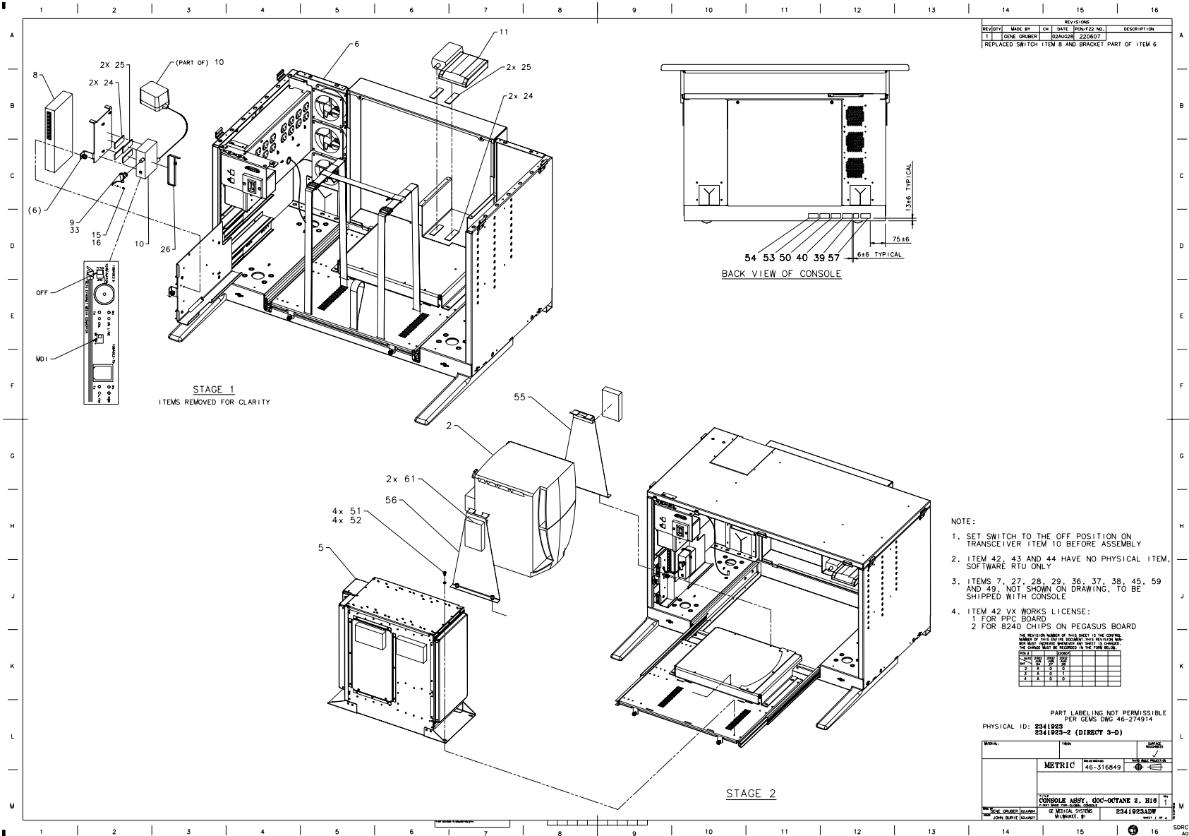
Figure 5-2 Console (2341923, sheet 1, rev 1)
