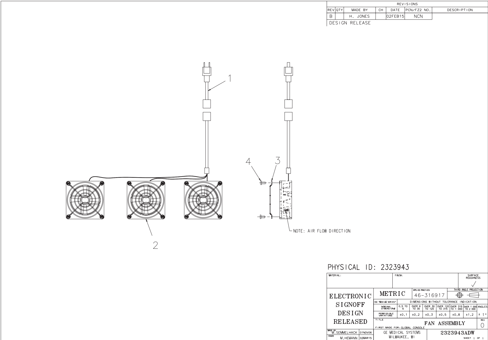
Figure 5-25 Fan Assembly, Console Chassis (2323943, sheet 1, rev 0)
