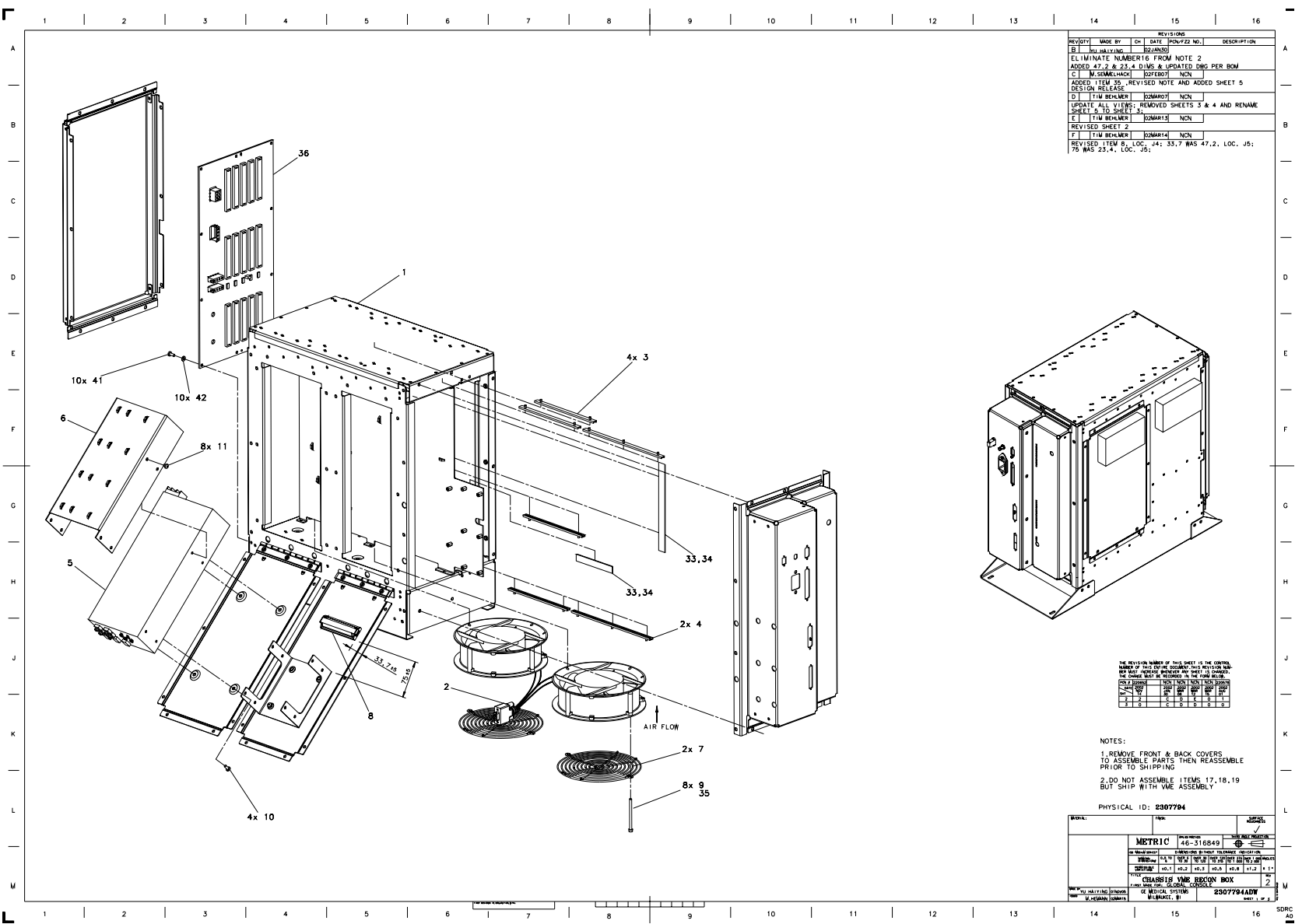
Figure 5-18 VME Chassis Assembly (2307794, sheet 1, rev 2)
