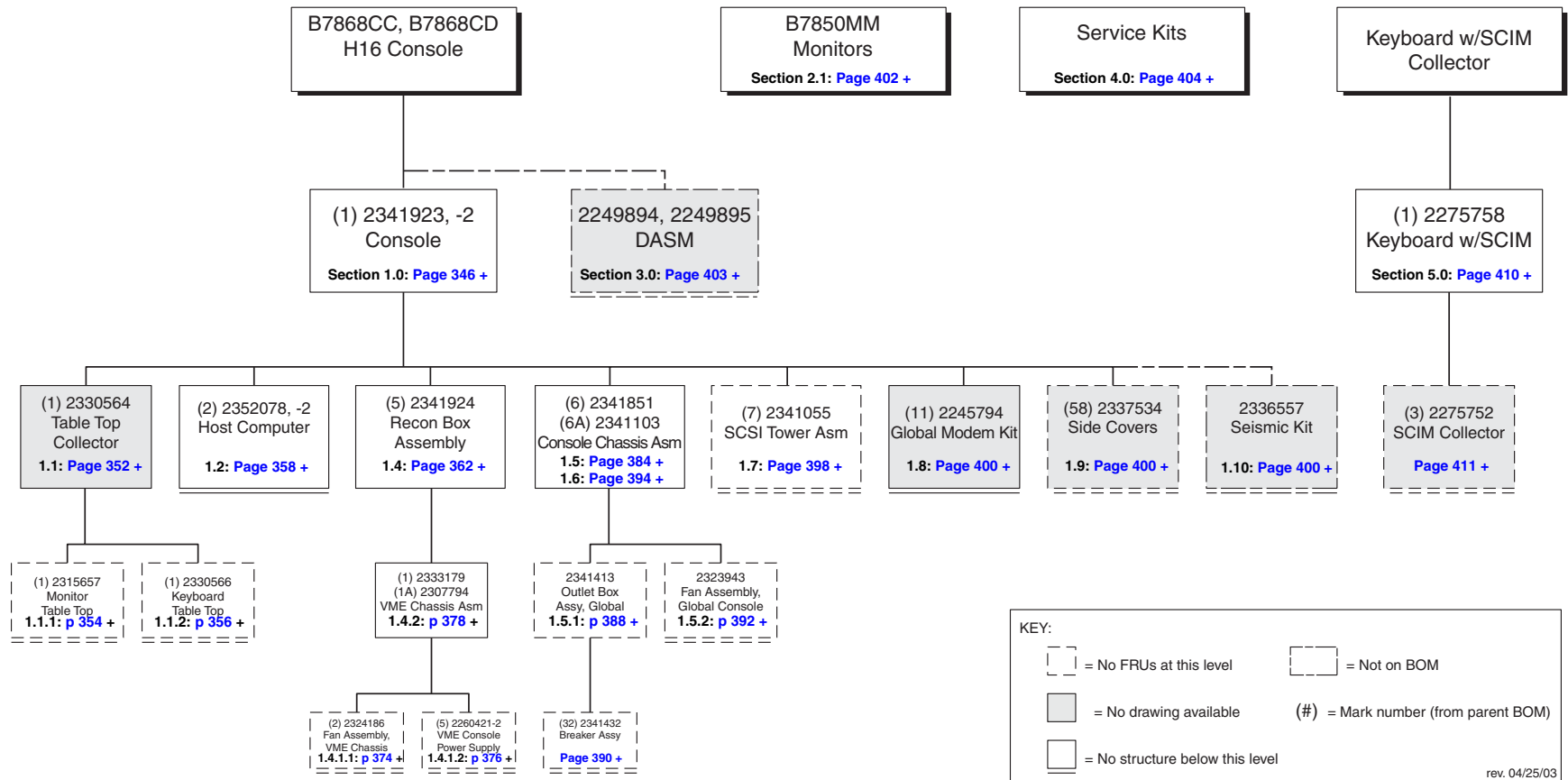
Figure 5-1 H16 Console (GOC1), BOM Tree
