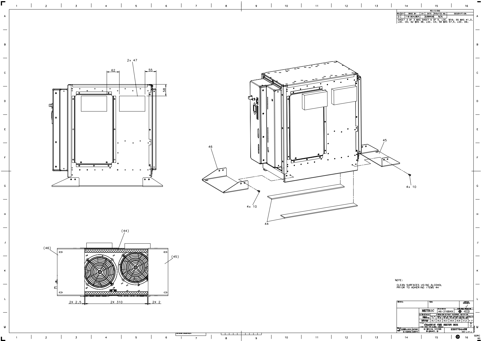
Figure 5-20 VME Chassis Assembly (2307794, sheet 3, rev 0)
