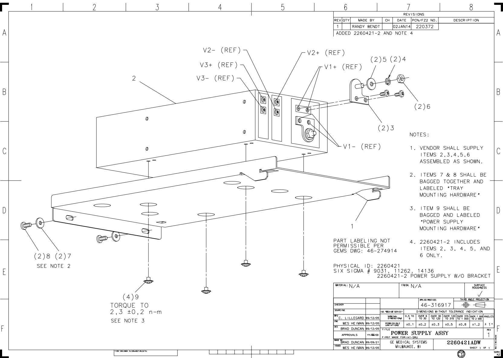
Figure 5-17 VME Console Power Supply (2260421, sheet 1, rev 1)
