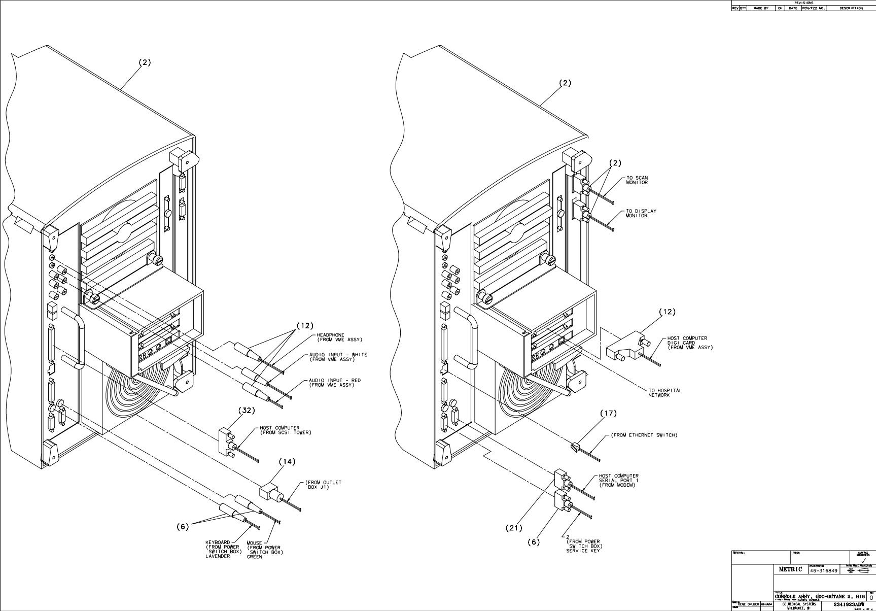
Figure 5-5 Console (2341923, sheet 4, rev 0)
