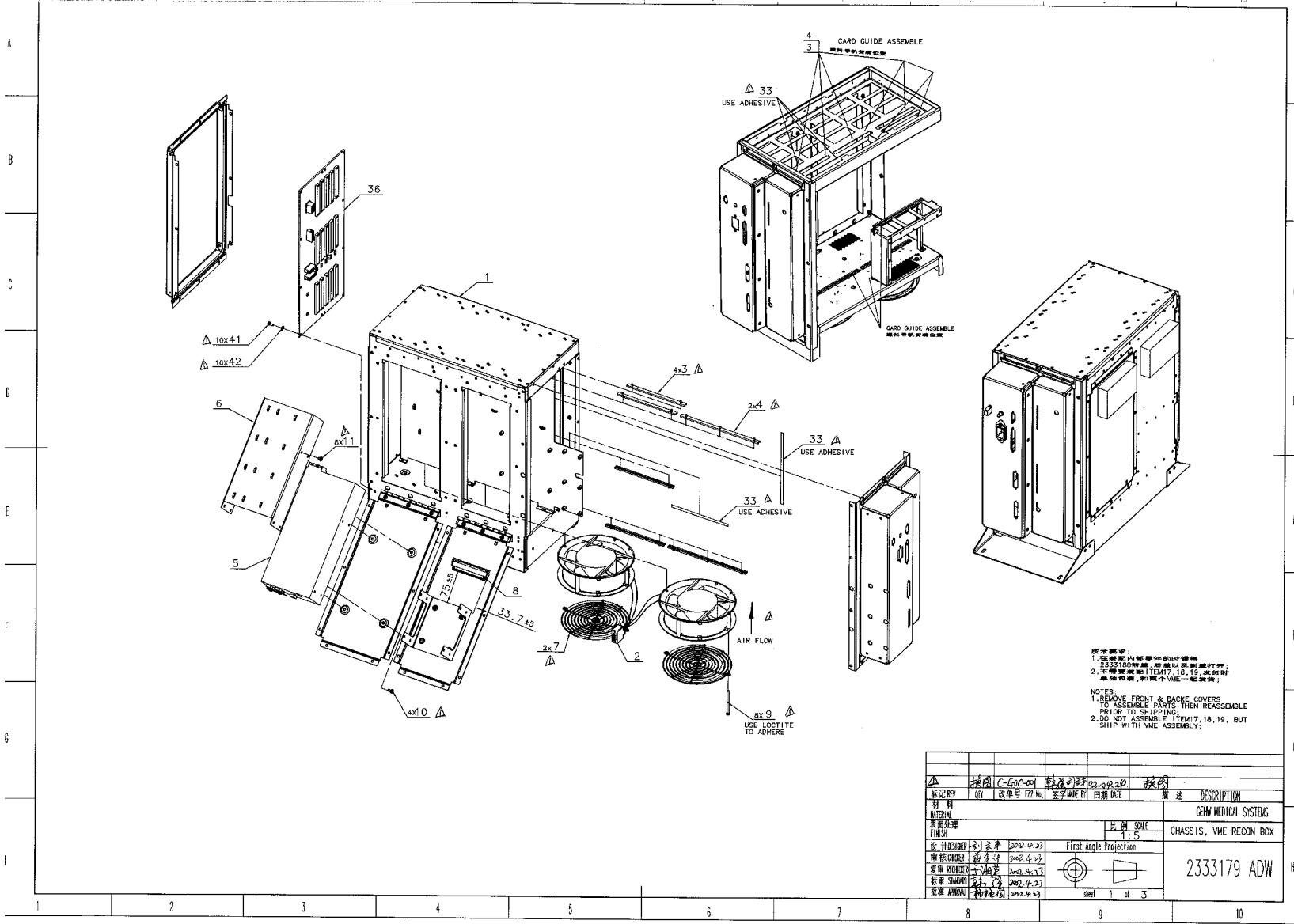
Figure 5-13 VME Recon Box Chassis (2333179 sheet 1, rev 1)
